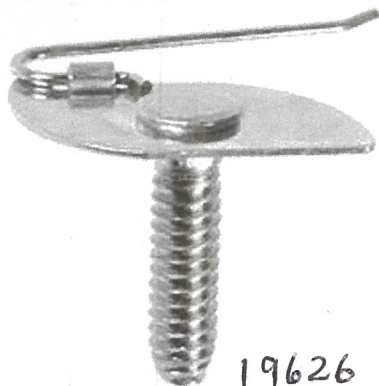
Universal Moulding Fastener #10-24 X 3/4 Bolt
