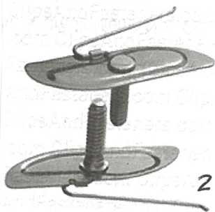
1-25/32" X 9/16" Universal Moulding Fastener #10-24 X 3/4" Bolt
