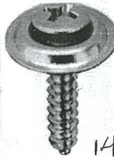
#8 X 1-1/2" Phillips Oval #6 Head Sems Countersunk Washer Chrome
