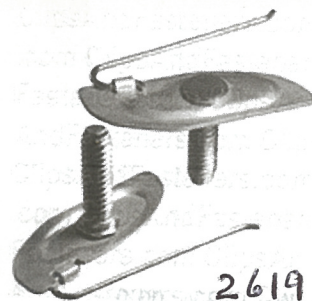
1-11/32" X 1/2" Universal Moulding Fastener #10-24 X 3/4" Bolt
