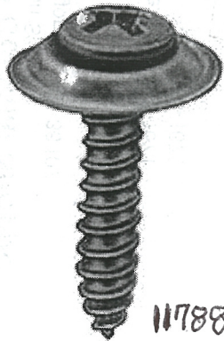
#8 X 3/4" Phillips Oval #6 Head Sems Countersunk Washer Black Phosphate
