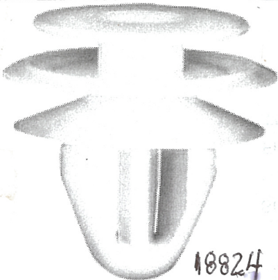
Mazda & Ford Trim Panel Retainer 9.5mm Stem Length
